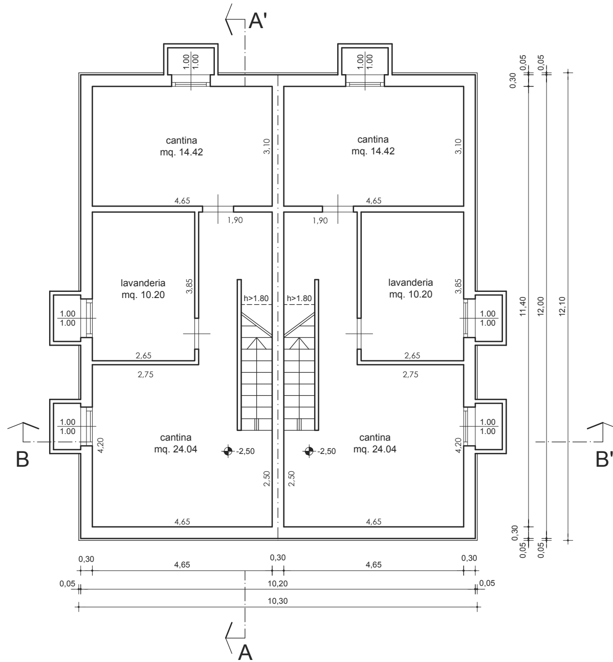
PIANO INTERRATO
